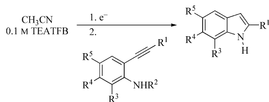
Scheme 1. Electrochemical-mediated cyclization of 2-alkynylanilines.
